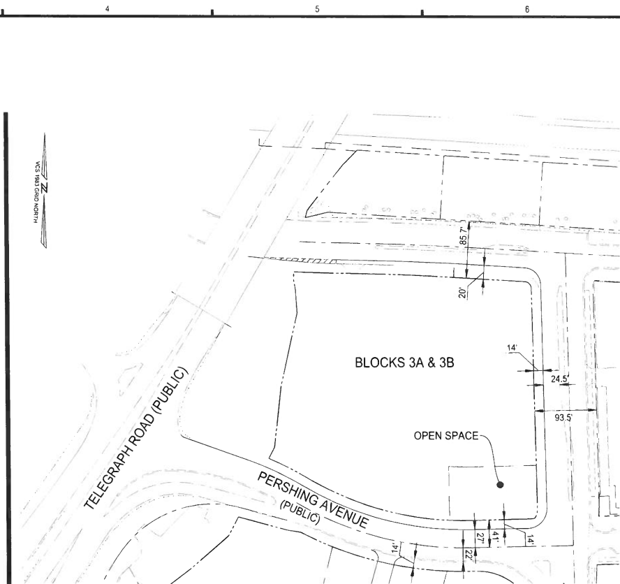
BLOCK 3 LAYOUT - WITHOUT ROAD
